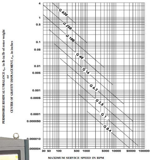
Figure 1-A Maximum permissible residual unbalance, e_{per} (Imperial values adapted from ISO 1940/1)
